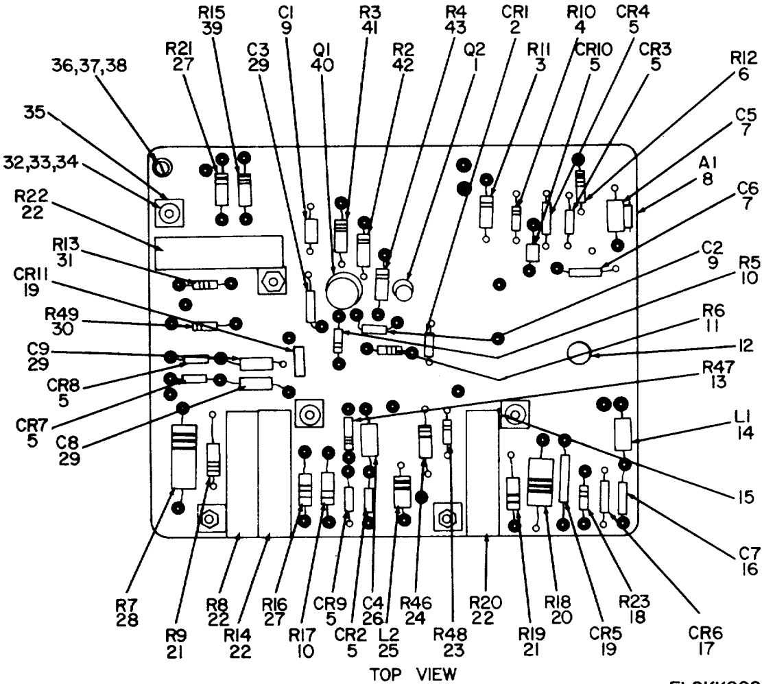
Figure 7. Function Board.
