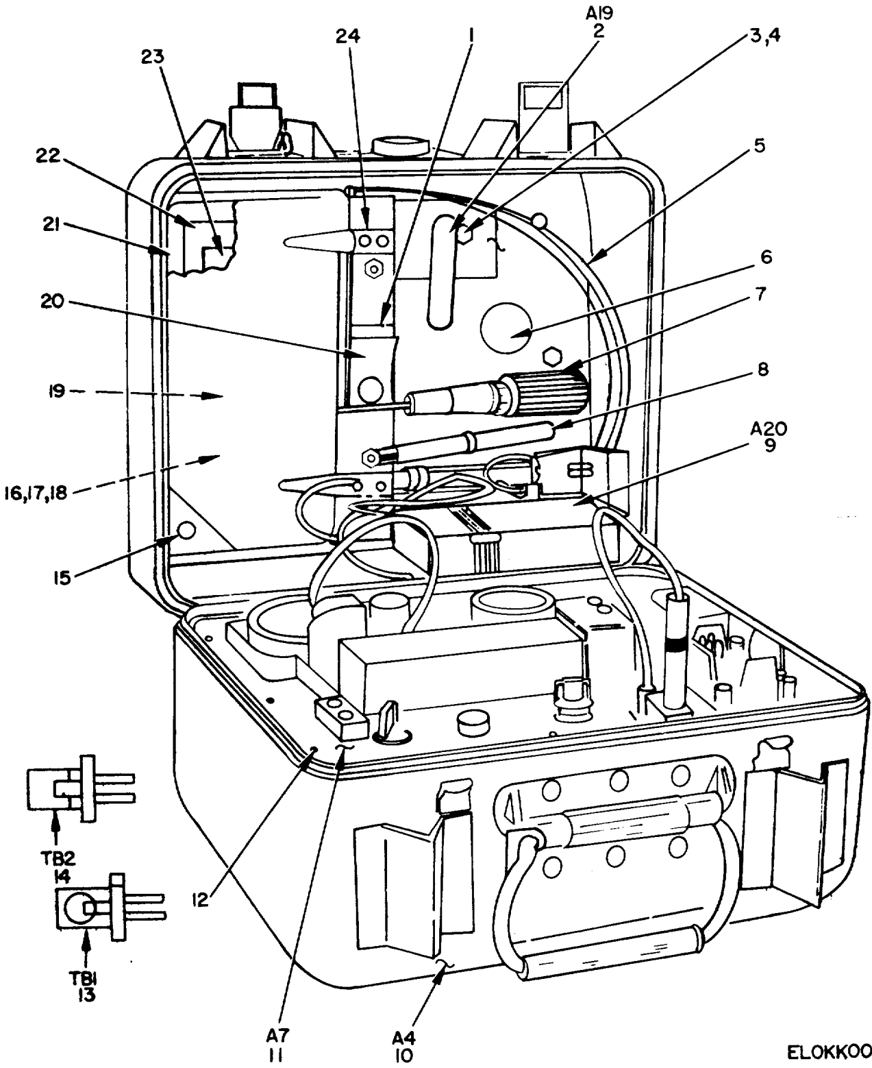
Figure 1. Indicators, Channel Alignment ID-1189/PR and ID-1189(XE-2)/PR.
