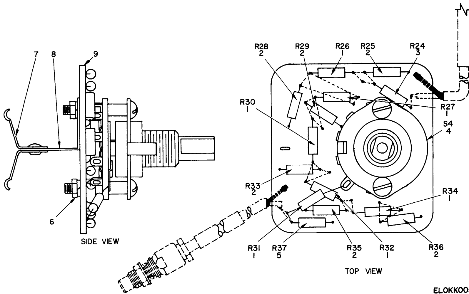
Figure 4. Attenuator Board Assembly
