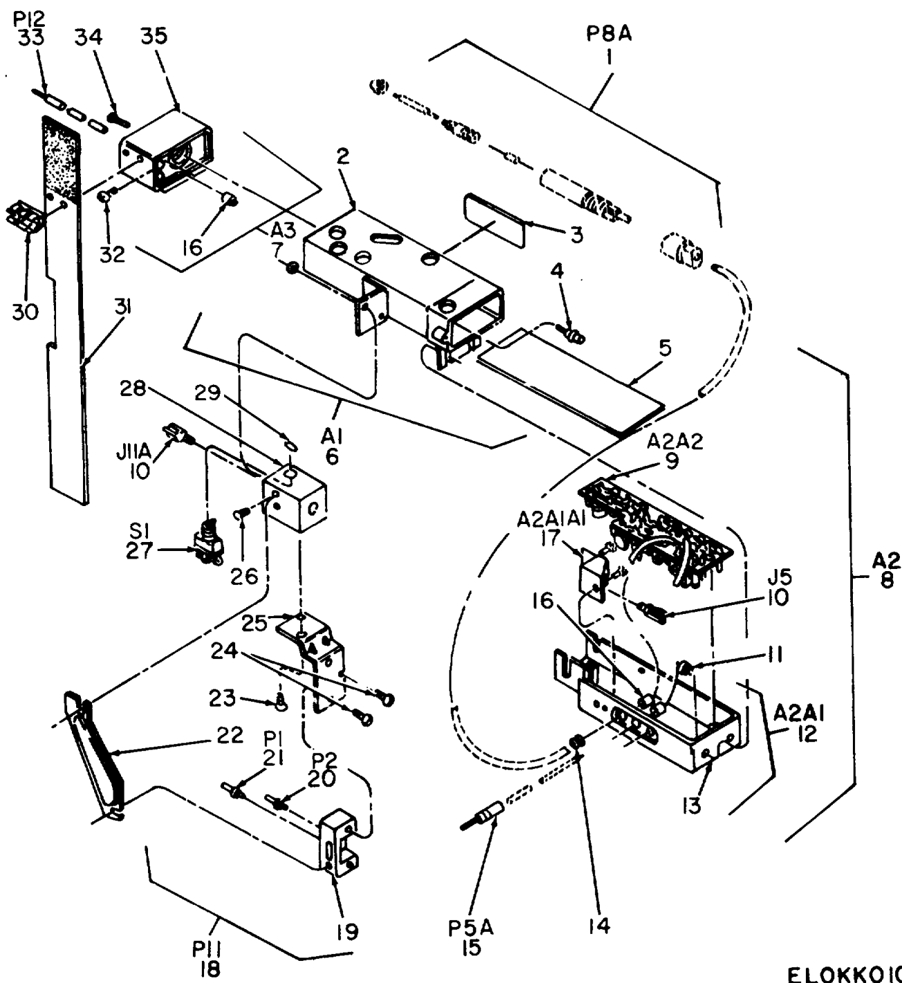
Figure 9. Adapter, Receiving Set MX-8512(XE-1)/PR.
