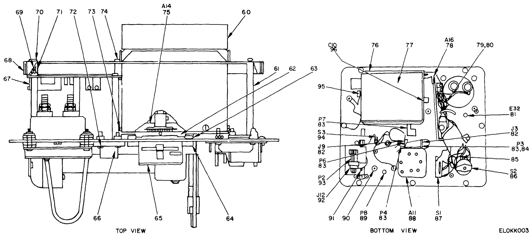
Figure 2. Top Plate Assembly (Sheet 2 of 2).
