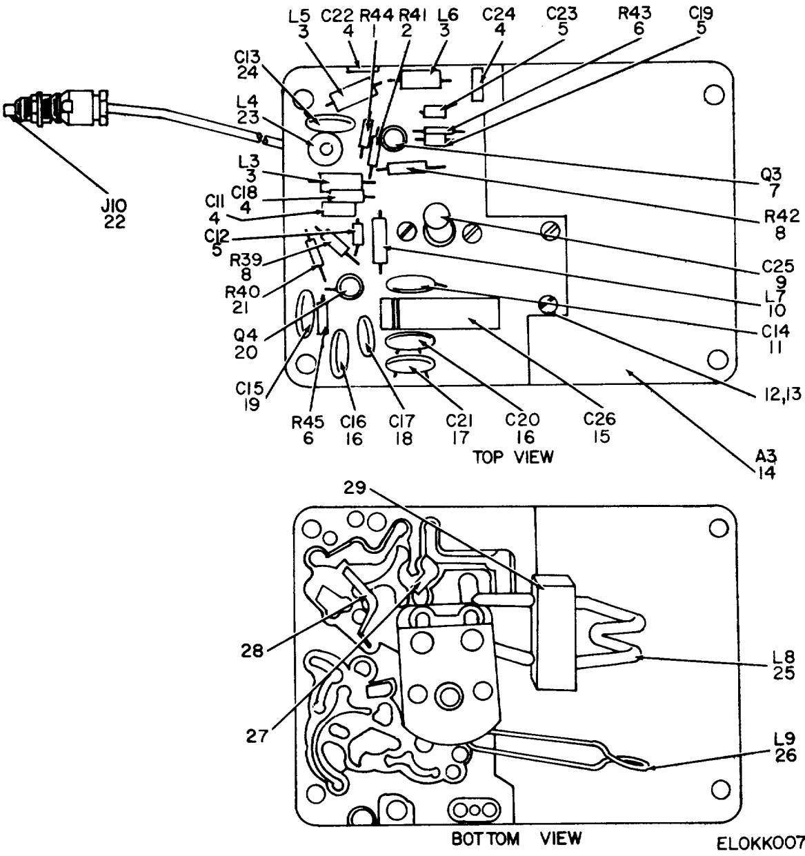
Figure 6. Board Assembly: VFO.
