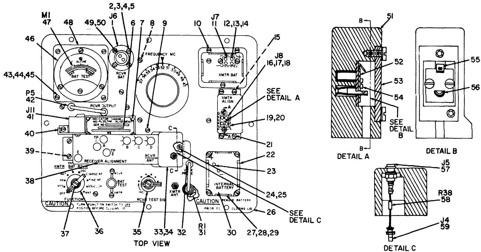
Figure 2. Top Plate Assembly (Sheet 1 of 2).
