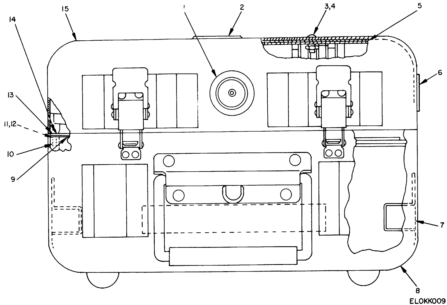
Figure 8. Case CY-6078/PR.
