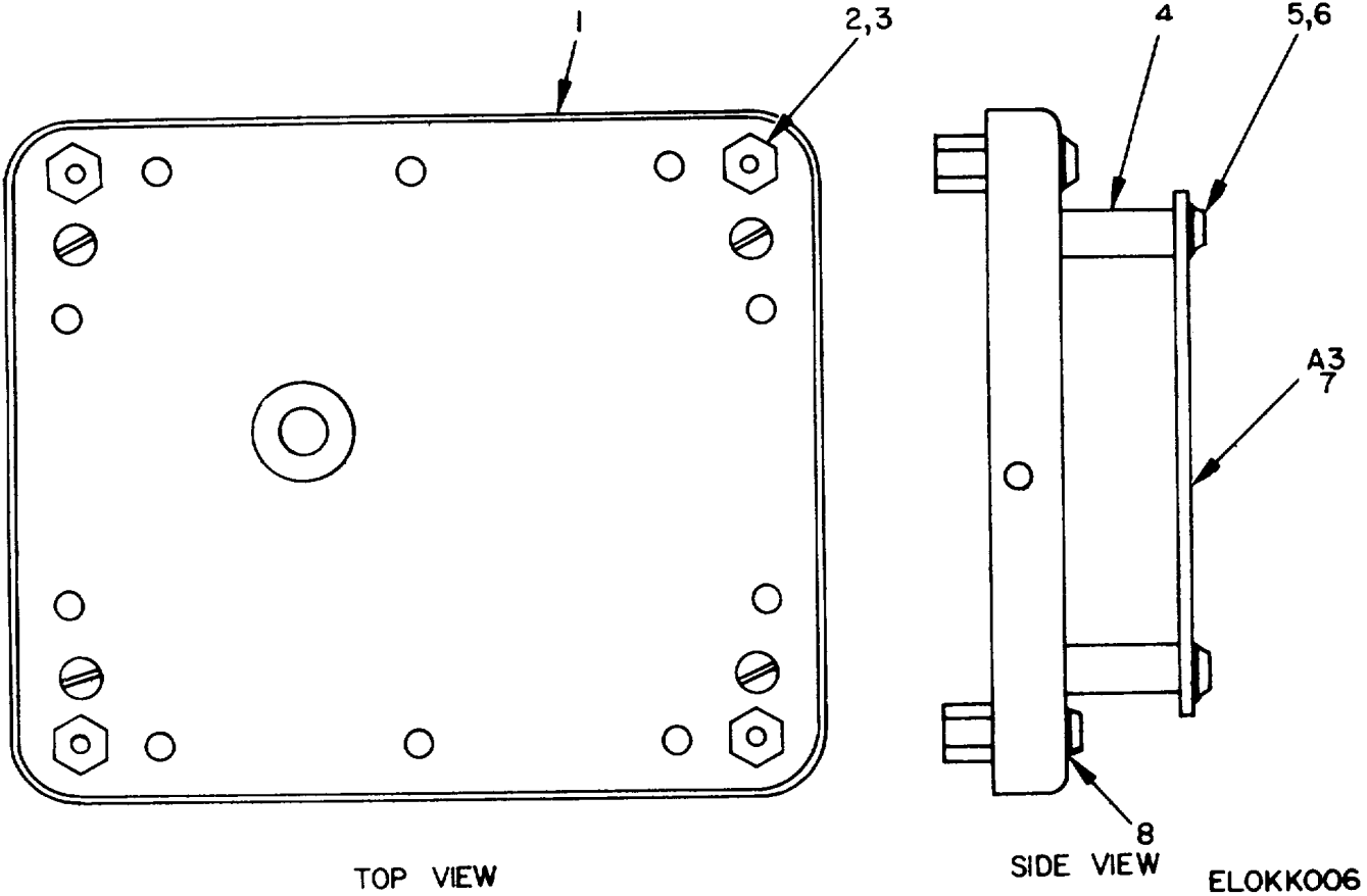
Figure 5. Shield Assembly: VFO.
